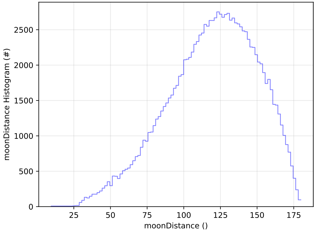
ddf_acor_sf10_lsf20_lsr50_v3.4_10yrs WFD u band: moonDistance Histogram
