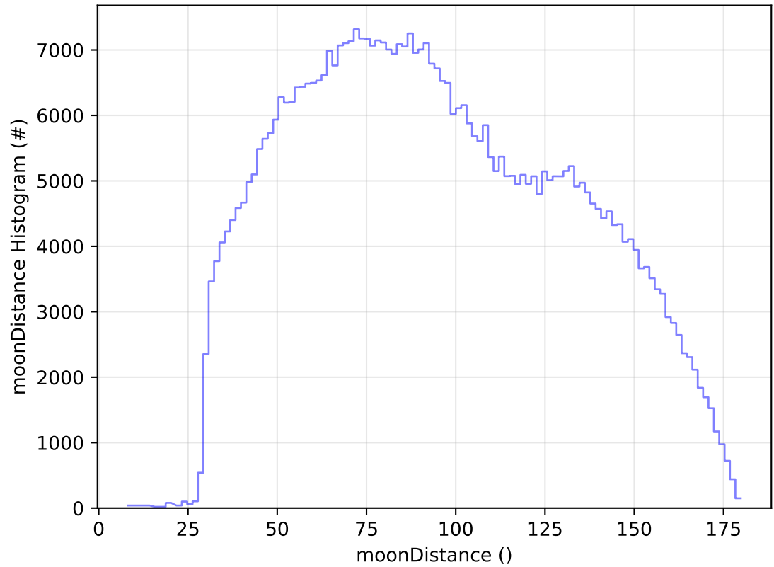
ddf_acor_sf10_lsf20_lsr50_v3.4_10yrs WFD i band: moonDistance Histogram
