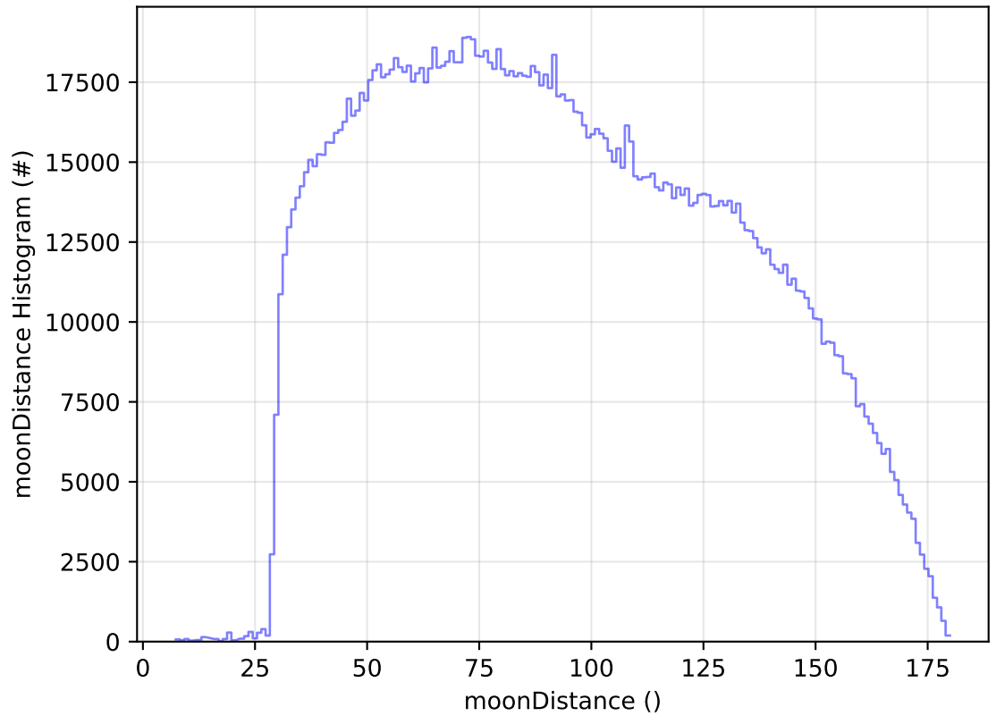
ddf_acor_sf10_lsf20_lsr50_v3.4_10yrs WFD all bands: moonDistance Histogram
