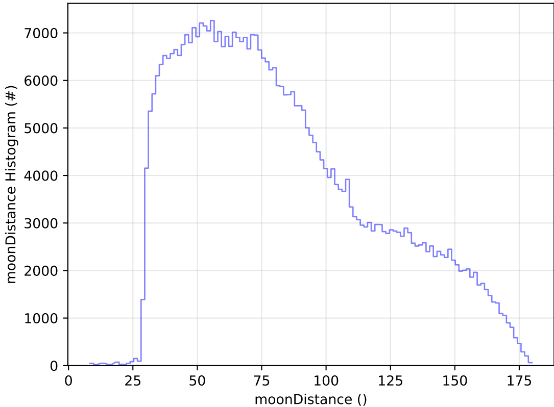
ddf_acor_sf10_lsf20_lsr50_v3.4_10yrs All sky z band: moonDistance Histogram
