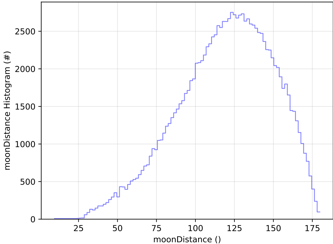
ddf_acor_sf10_lsf20_lsr50_v3.4_10yrs All sky u band: moonDistance Histogram
