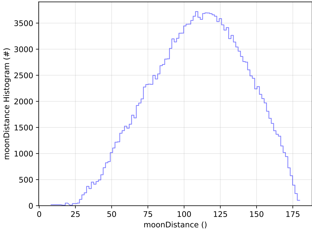
ddf_acor_sf10_lsf20_lsr50_v3.4_10yrs All sky g band: moonDistance Histogram
