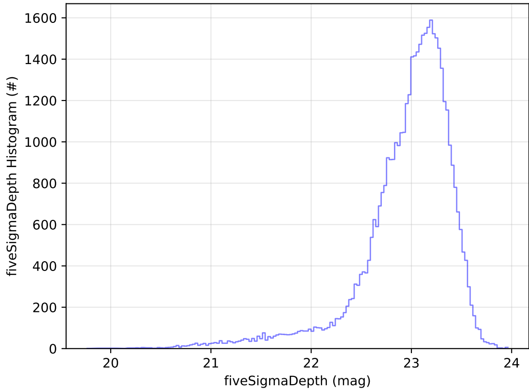
ddf_acor_sf10_lsf20_lsr50_v3.4_10yrs Yr 1 z band: fiveSigmaDepth Histogram
