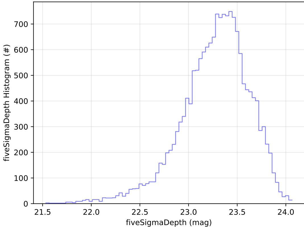
ddf_acor_sf10_lsf20_lsr50_v3.4_10yrs Yr 1 u band: fiveSigmaDepth Histogram
