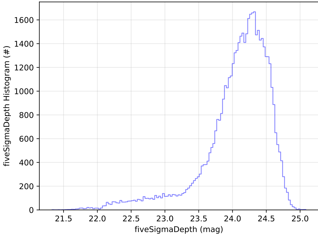
ddf_acor_sf10_lsf20_lsr50_v3.4_10yrs Yr 1 r band: fiveSigmaDepth Histogram
