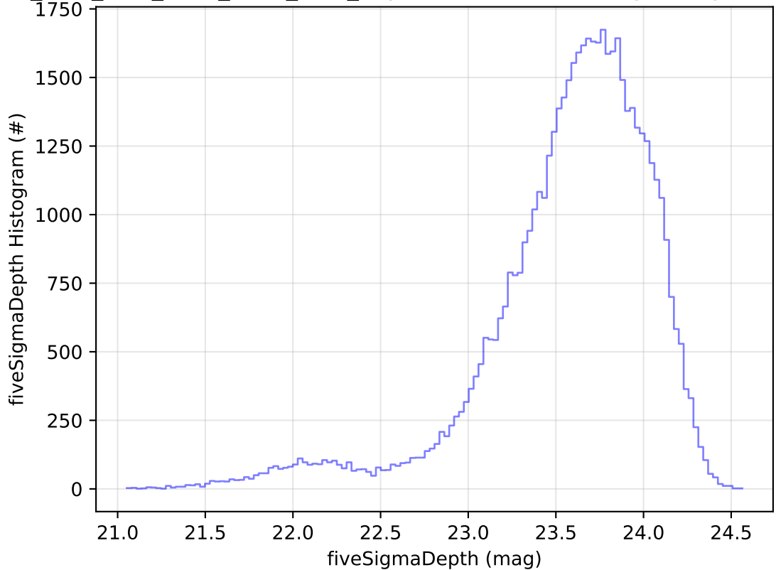
ddf_acor_sf10_lsf20_lsr50_v3.4_10yrs Yr 1 i band: fiveSigmaDepth Histogram
