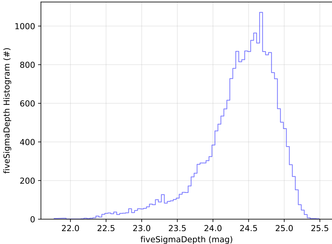
ddf_acor_sf10_lsf20_lsr50_v3.4_10yrs Yr 1 g band: fiveSigmaDepth Histogram
