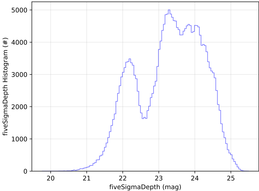
ddf_acor_sf10_lsf20_lsr50_v3.4_10yrs Yr 1 all bands: fiveSigmaDepth Histogram
