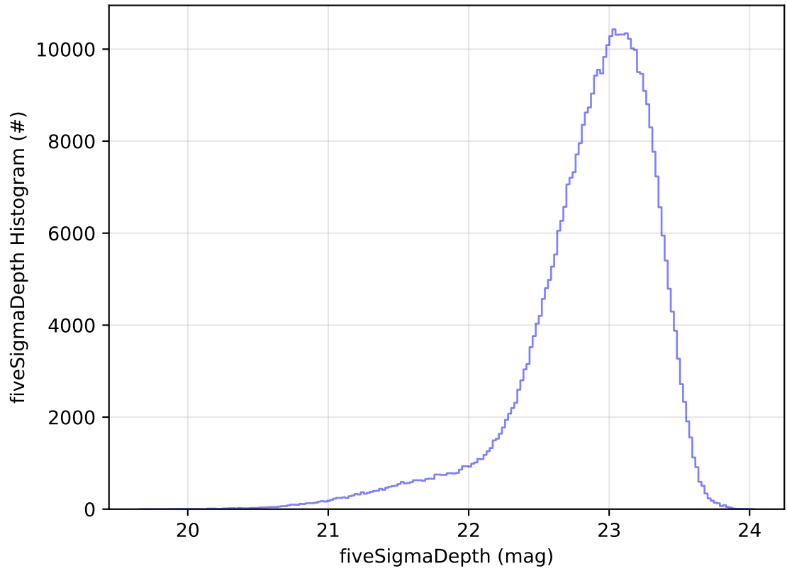
ddf_acor_sf10_lsf20_lsr50_v3.4_10yrs WFD z band: fiveSigmaDepth Histogram
