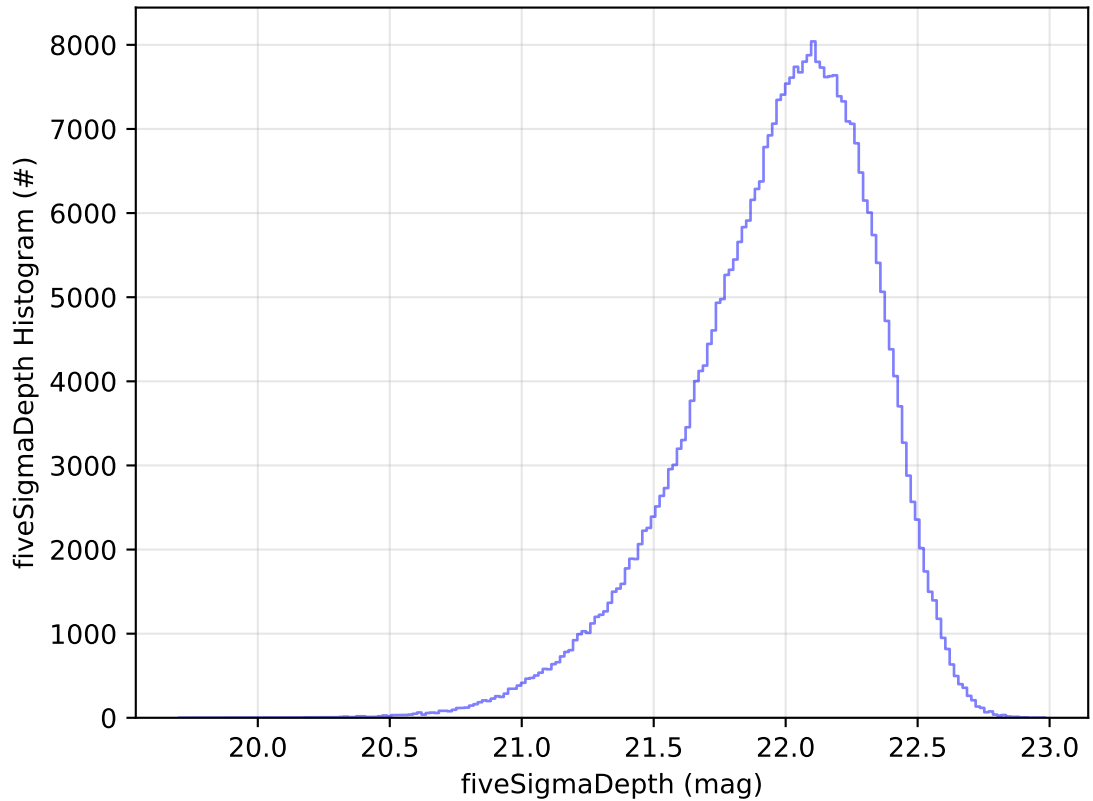
ddf_acor_sf10_lsf20_lsr50_v3.4_10yrs WFD y band: fiveSigmaDepth Histogram
