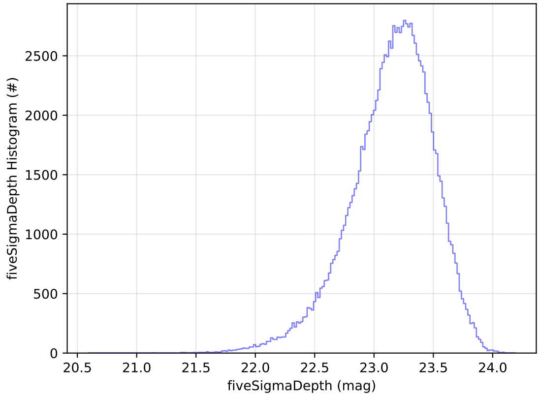
ddf_acor_sf10_lsf20_lsr50_v3.4_10yrs WFD u band: fiveSigmaDepth Histogram
