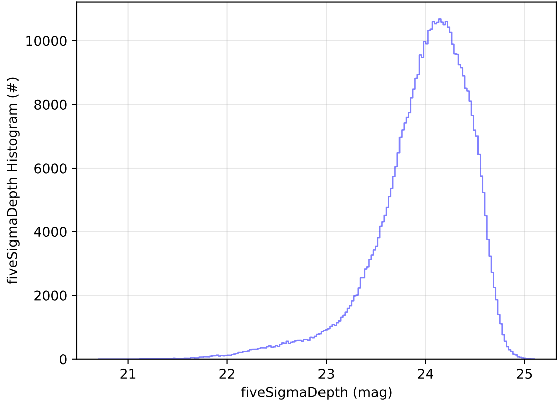
ddf_acor_sf10_lsf20_lsr50_v3.4_10yrs WFD r band: fiveSigmaDepth Histogram
