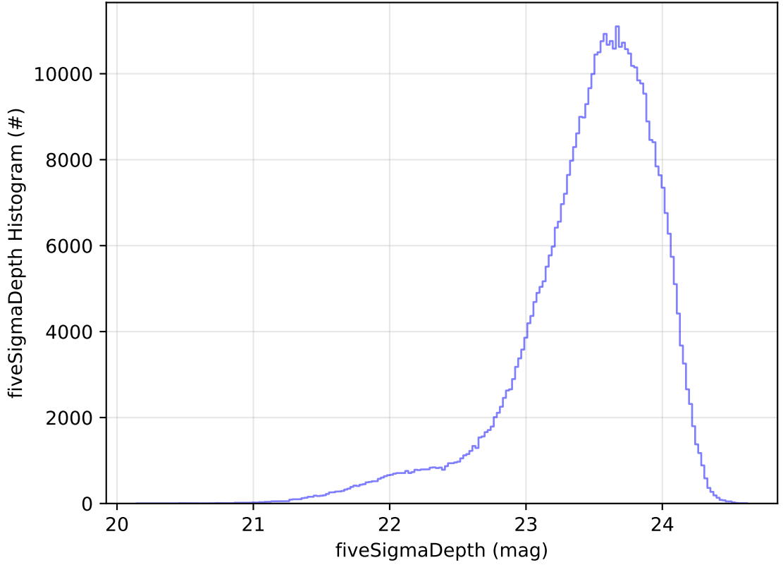
ddf_acor_sf10_lsf20_lsr50_v3.4_10yrs WFD i band: fiveSigmaDepth Histogram
