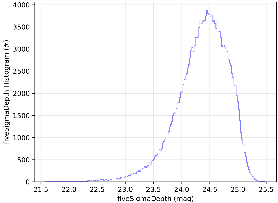
ddf_acor_sf10_lsf20_lsr50_v3.4_10yrs WFD g band: fiveSigmaDepth Histogram
