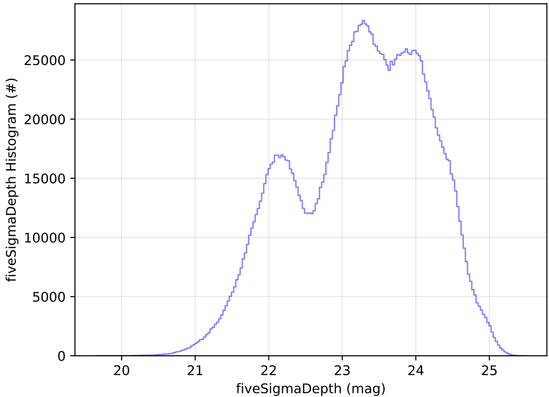
ddf_acor_sf10_lsf20_lsr50_v3.4_10yrs WFD all bands: fiveSigmaDepth Histogram
