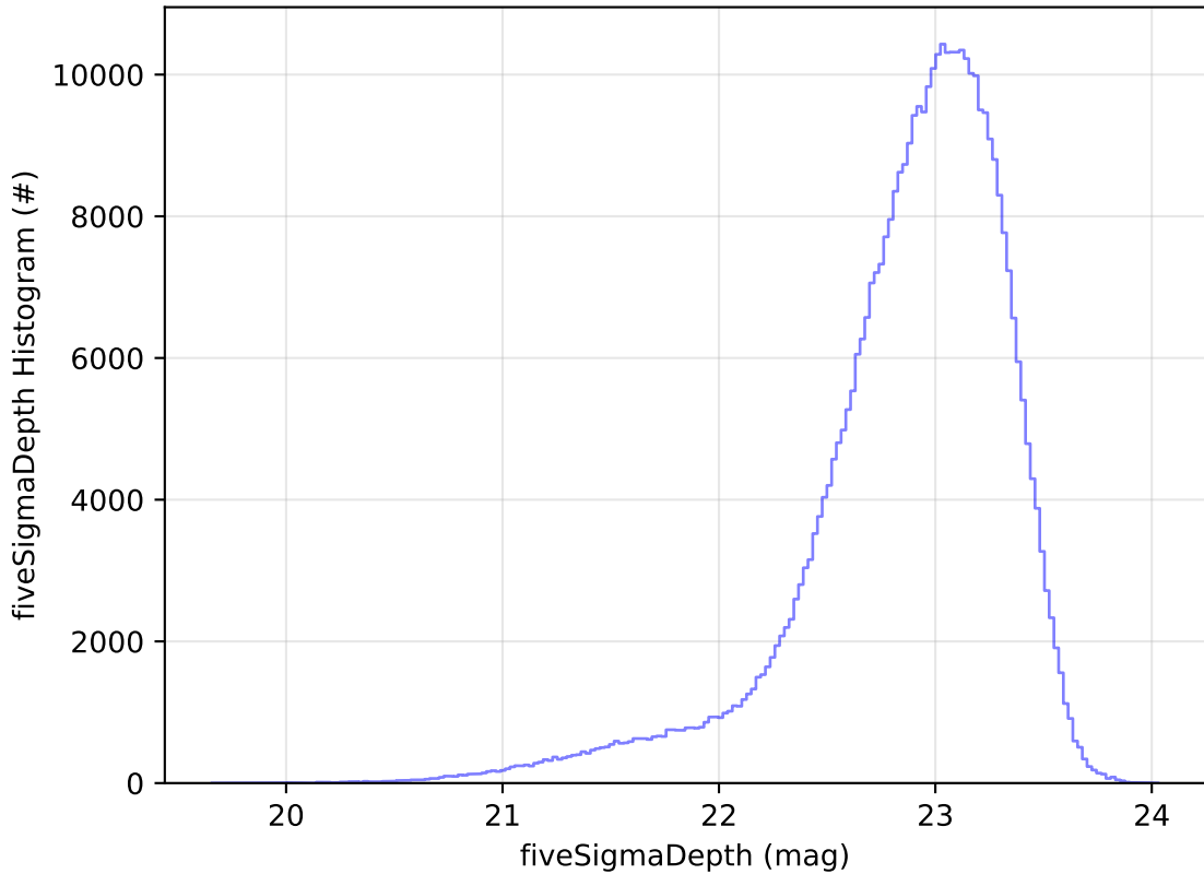
ddf_acor_sf10_lsf20_lsr50_v3.4_10yrs All sky z band: fiveSigmaDepth Histogram
