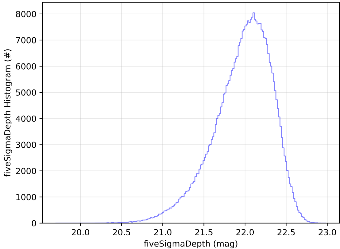
ddf_acor_sf10_lsf20_lsr50_v3.4_10yrs All sky y band: fiveSigmaDepth Histogram
