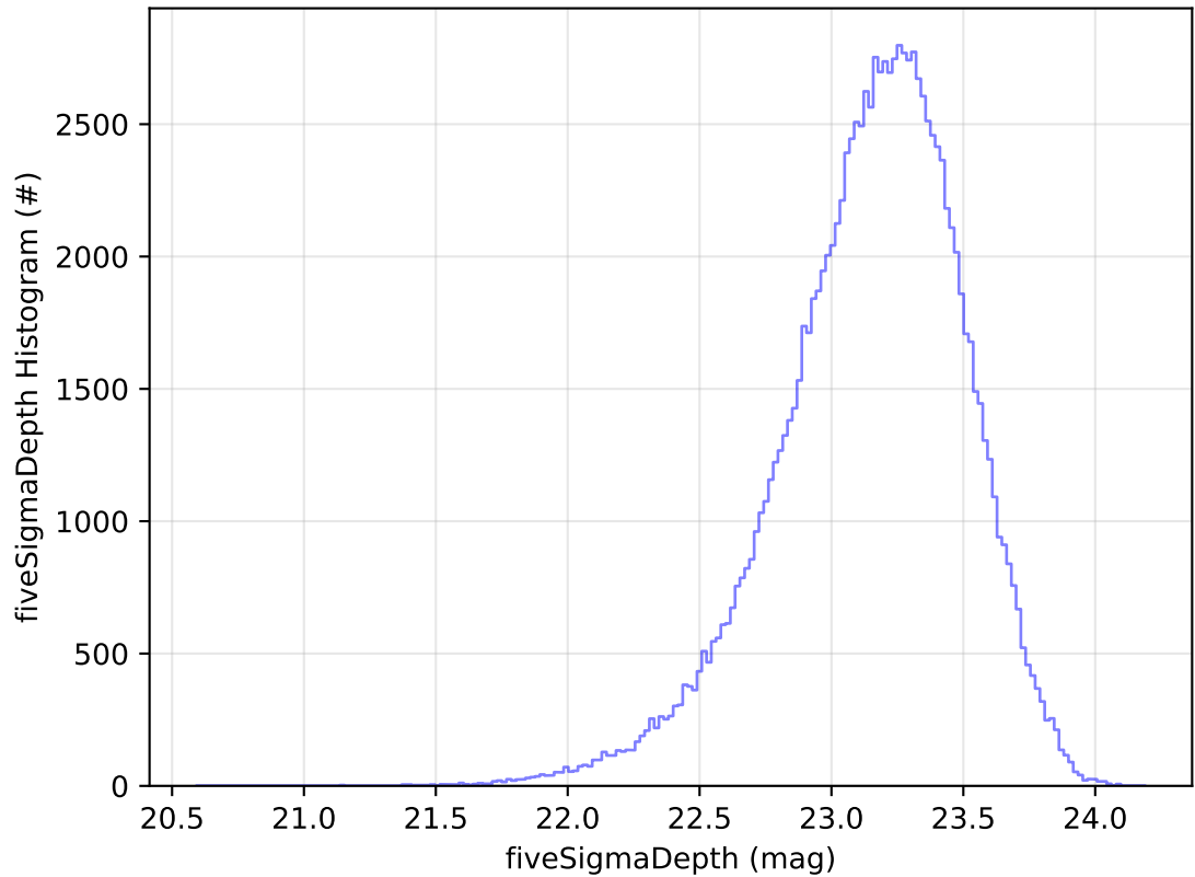
ddf_acor_sf10_lsf20_lsr50_v3.4_10yrs All sky u band: fiveSigmaDepth Histogram
