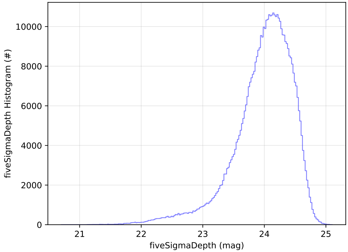
ddf_acor_sf10_lsf20_lsr50_v3.4_10yrs All sky r band: fiveSigmaDepth Histogram
