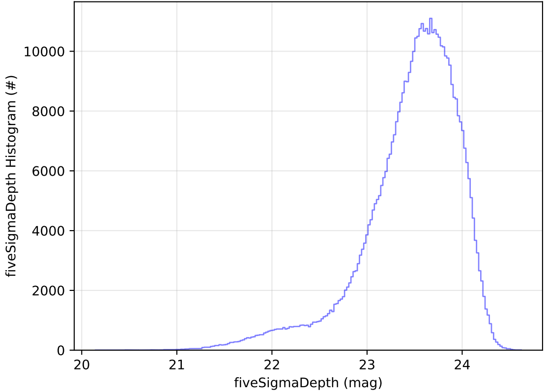
ddf_acor_sf10_lsf20_lsr50_v3.4_10yrs All sky i band: fiveSigmaDepth Histogram
