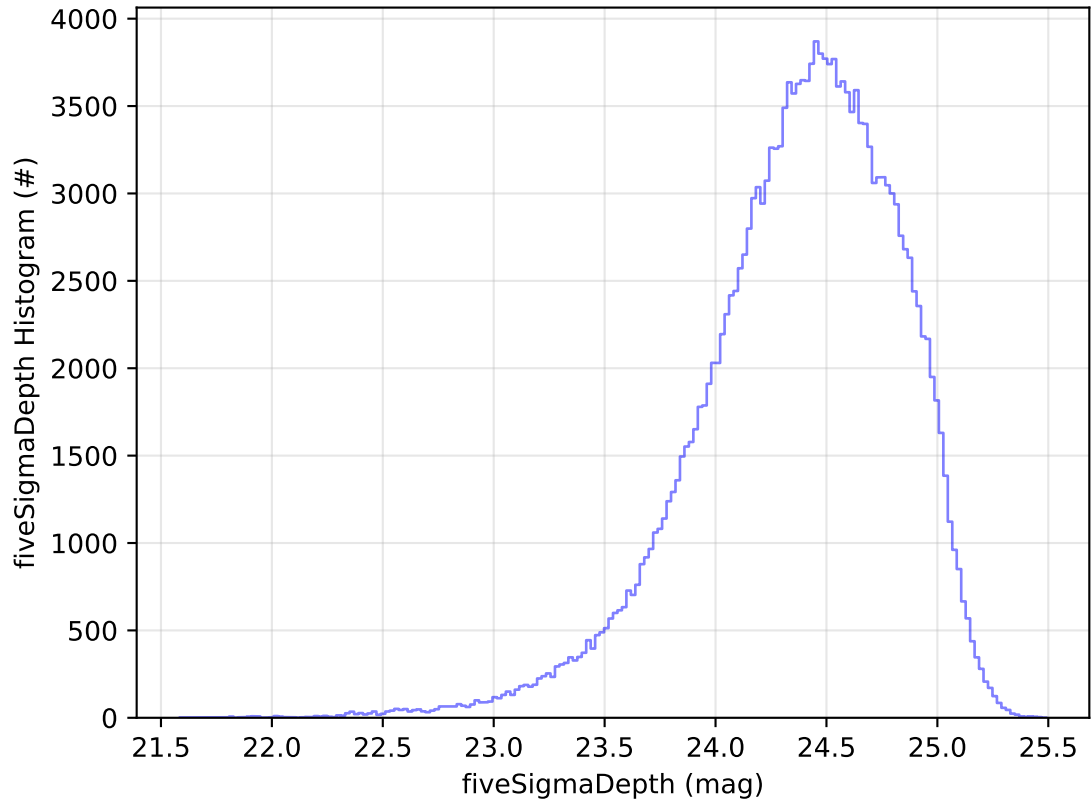
ddf_acor_sf10_lsf20_lsr50_v3.4_10yrs All sky g band: fiveSigmaDepth Histogram
