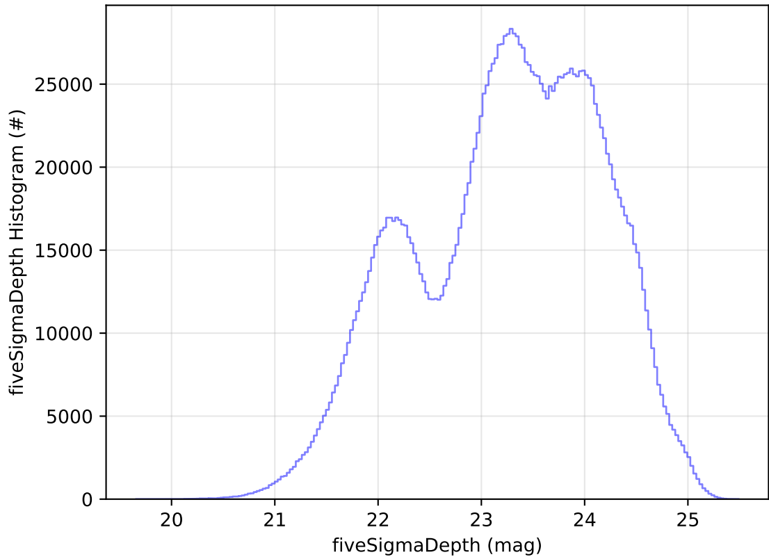
ddf_acor_sf10_lsf20_lsr50_v3.4_10yrs All sky all bands: fiveSigmaDepth Histogram
