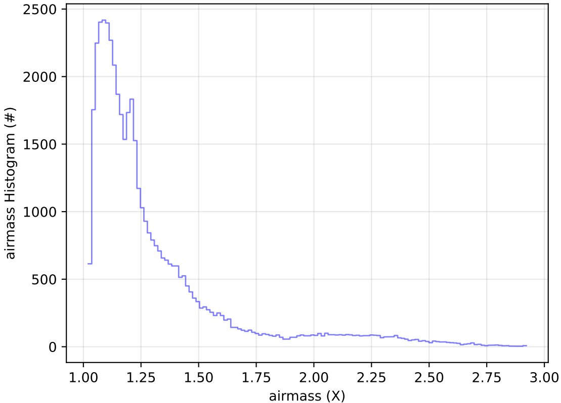
ddf_acor_sf10_lsf20_lsr50_v3.4_10yrs Yr 1 z band: airmass Histogram
