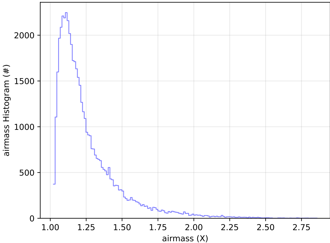
ddf_acor_sf10_lsf20_lsr50_v3.4_10yrs Yr 1 y band: airmass Histogram
