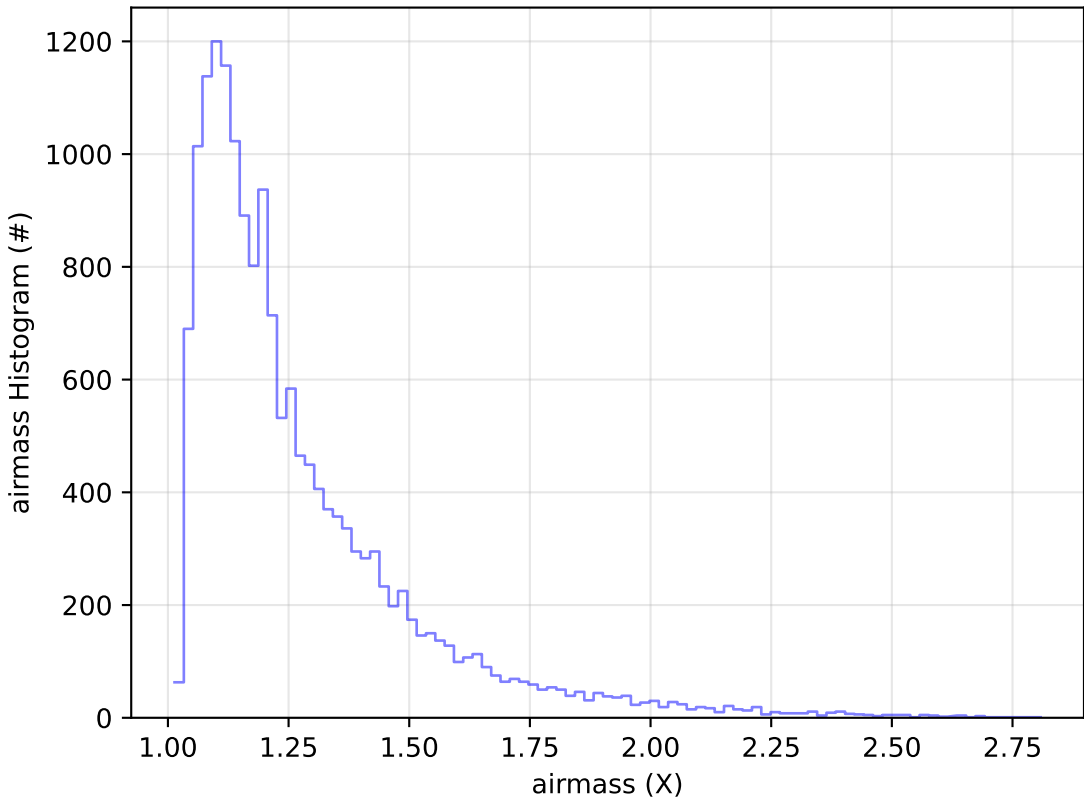
ddf_acor_sf10_lsf20_lsr50_v3.4_10yrs Yr 1 u band: airmass Histogram
