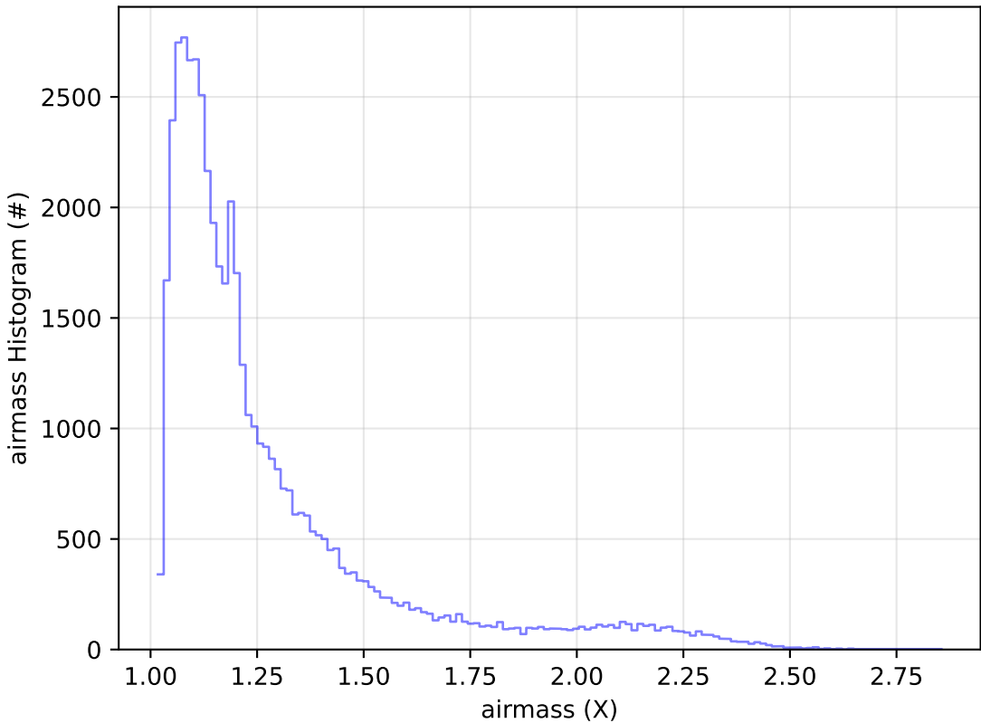
ddf_acor_sf10_ls20_lsr50_v3.4_10yrs Yr 1 r band: airmass Histogram
