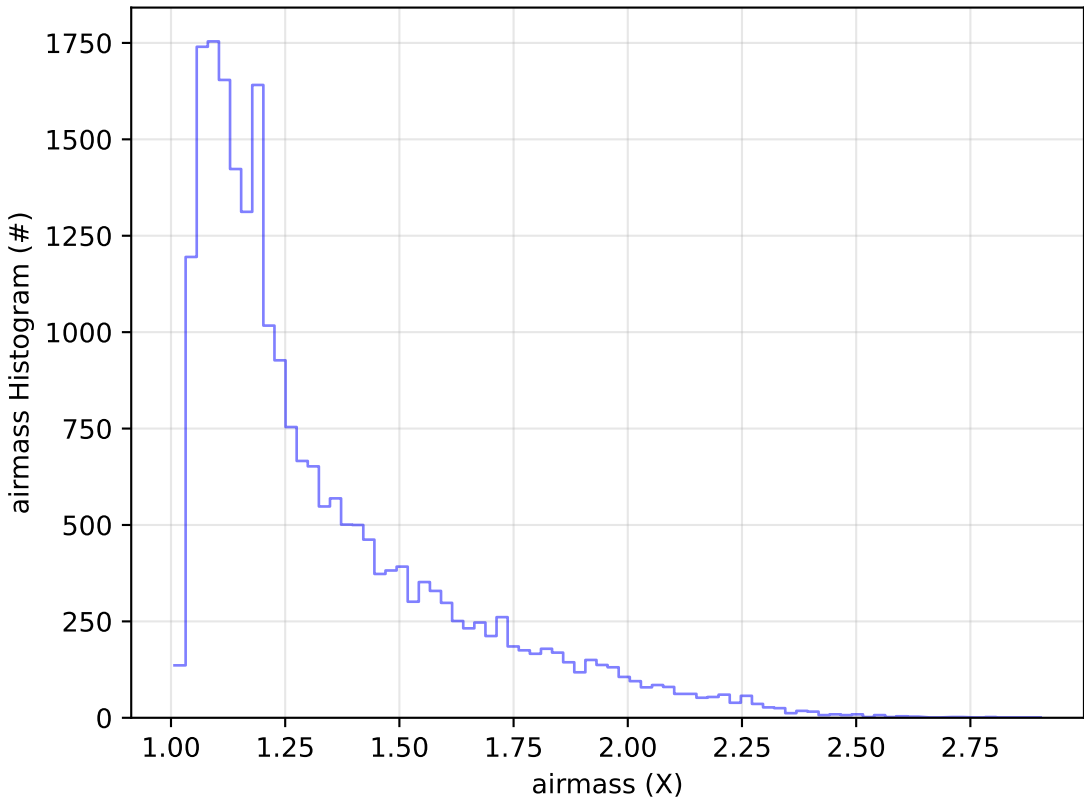
ddf_acor_sf10_lsf20_lsr50_v3.4_10yrs Yr 1 g band: airmass Histogram
