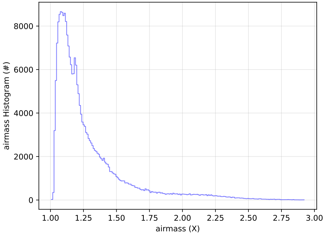
ddf_acor_sf10_lsf20_lsr50_v3.4_10yrs Yr 1 all bands: airmass Histogram
