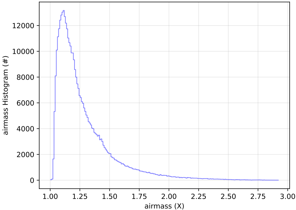
ddf_acor_sf10_lsf20_lsr50_v3.4_10yrs WFD y band: airmass Histogram
