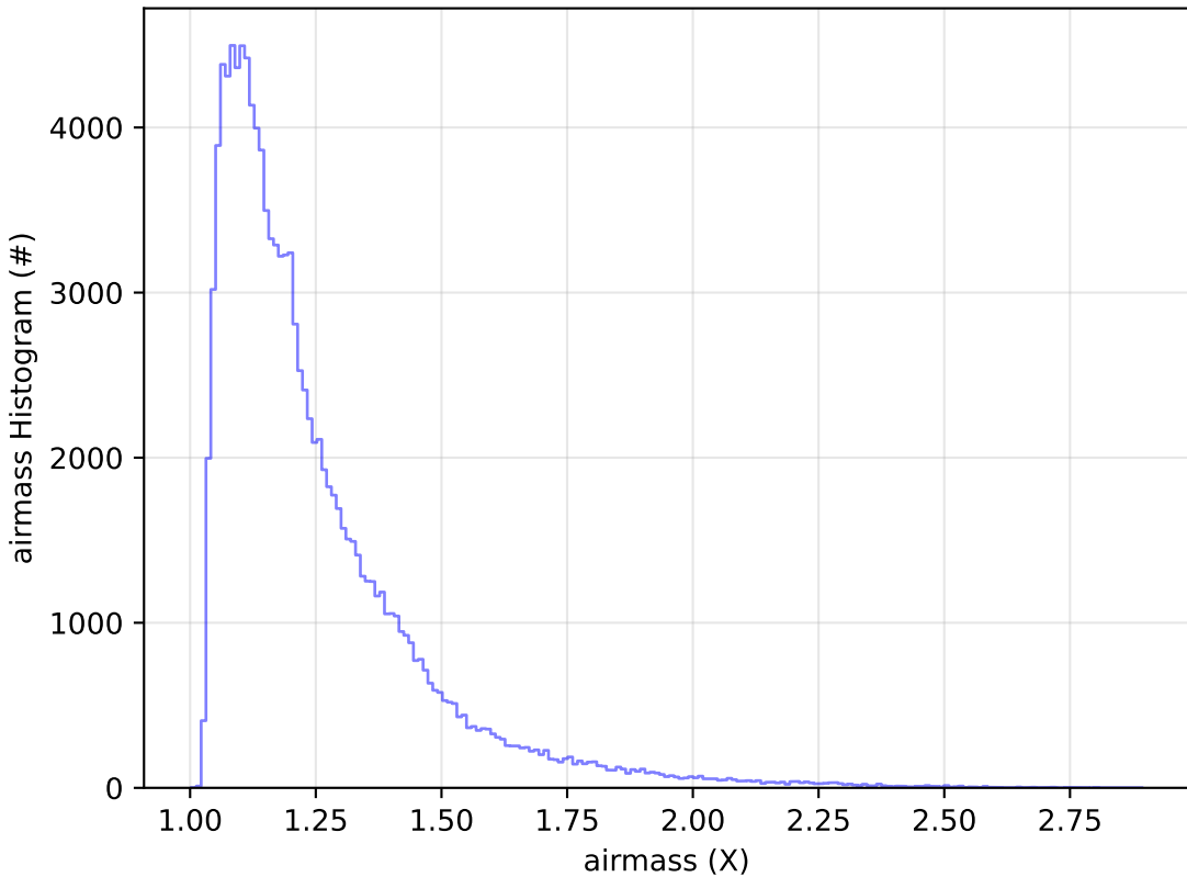
ddf_acor_sf10_lsf20_lsr50_v3.4_10yrs WFD u band: airmass Histogram
