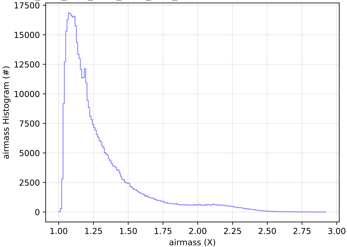
ddf_acor_sf10_lsf20_lsr50_v3.4_10yrs WFD r band: airmass Histogram
