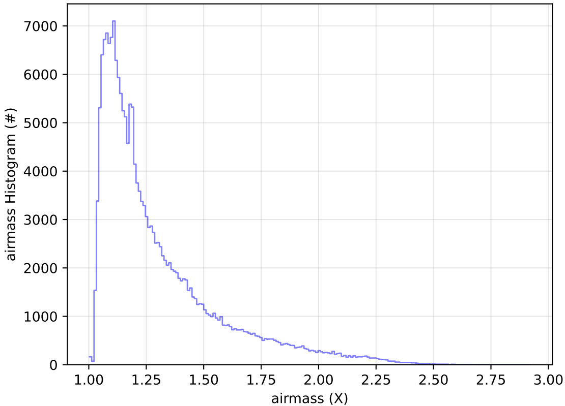
ddf_acor_sf10_lsf20_lsr50_v3.4_10yrs WFD g band: airmass Histogram
