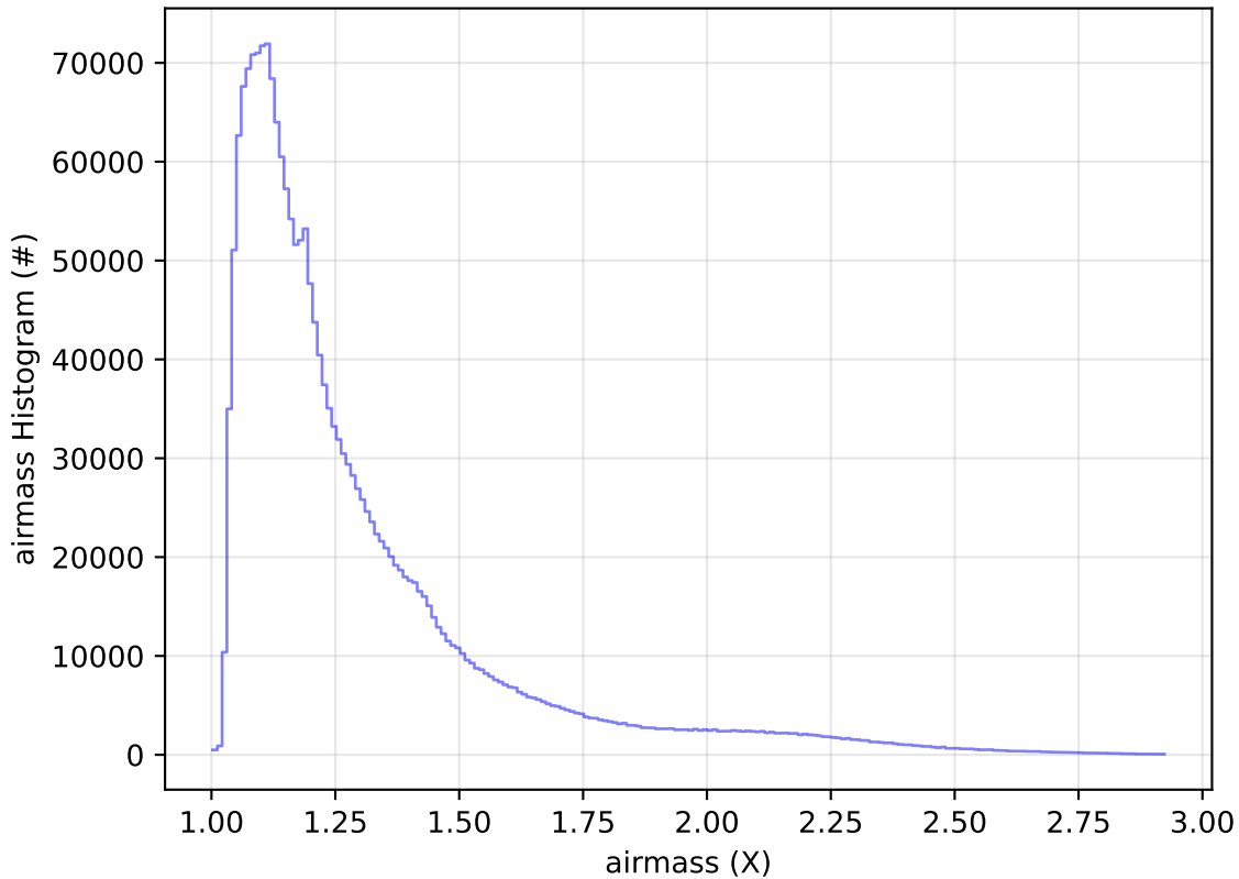
ddf_acor_sf10_lsf20_lsr50_v3.4_10yrs WFD all bands: airmass Histogram
