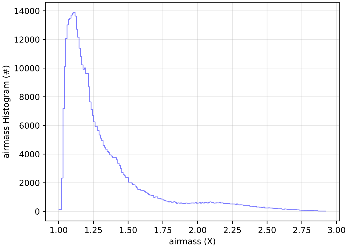
ddf_acor_sf10_lsf20_lsr50_v3.4_10yrs All sky z band: airmass Histogram
