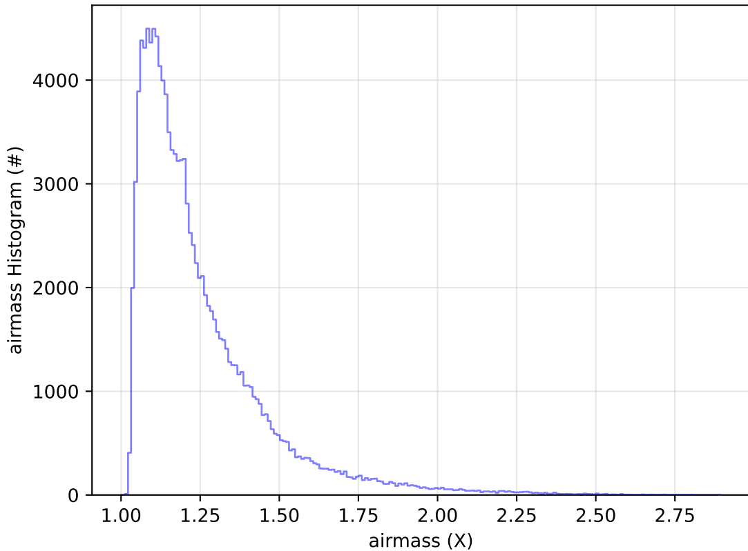
ddf_acor_sf10_lsf20_lsr50_v3.4_10yrs All sky u band: airmass Histogram
