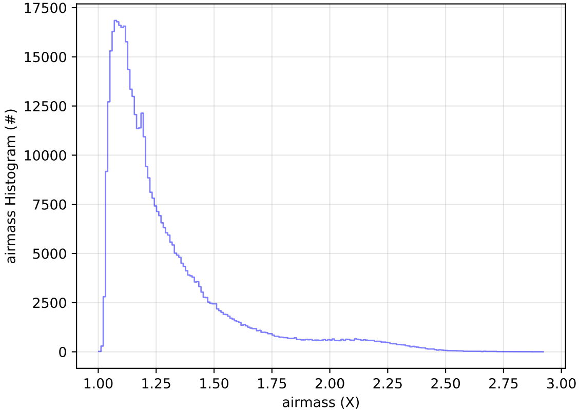
ddf_acor_sf10_lsf20_lsr50_v3.4_10yrs All sky r band: airmass Histogram
