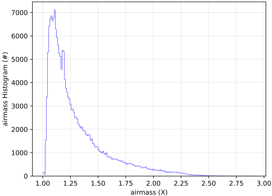
ddf_acor_sf10_lsf20_lsr50_v3.4_10yrs All sky g band: airmass Histogram
