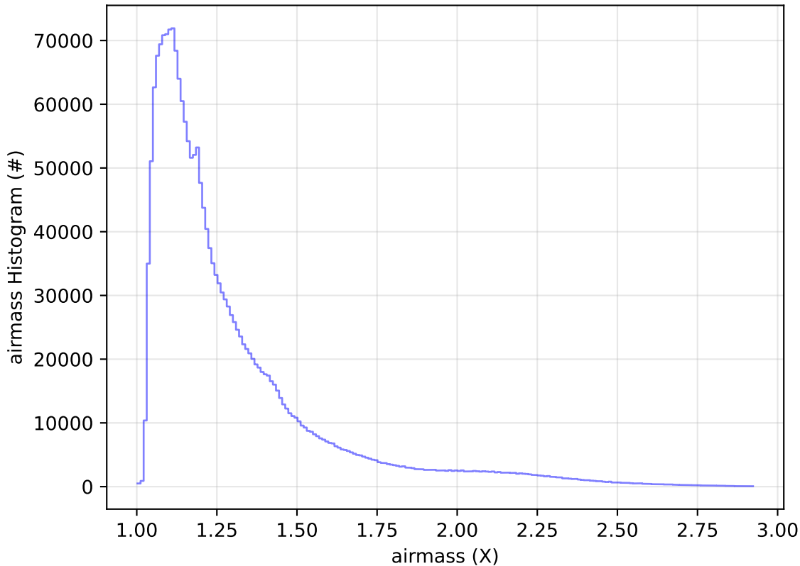
ddf_acor_sf10_lsf20_lsr50_v3.4_10yrs All sky all bands: airmass Histogram
