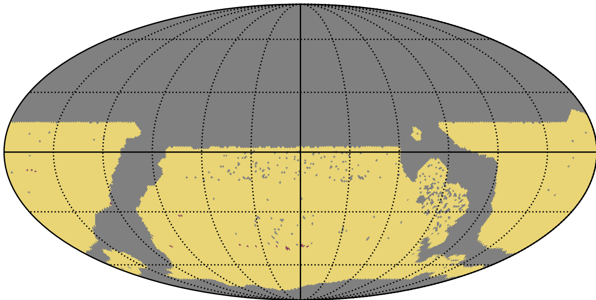
ddf_acor_sf10_lsf20_lsr50_v3.4_10yrs WFD: RapidRevisits
