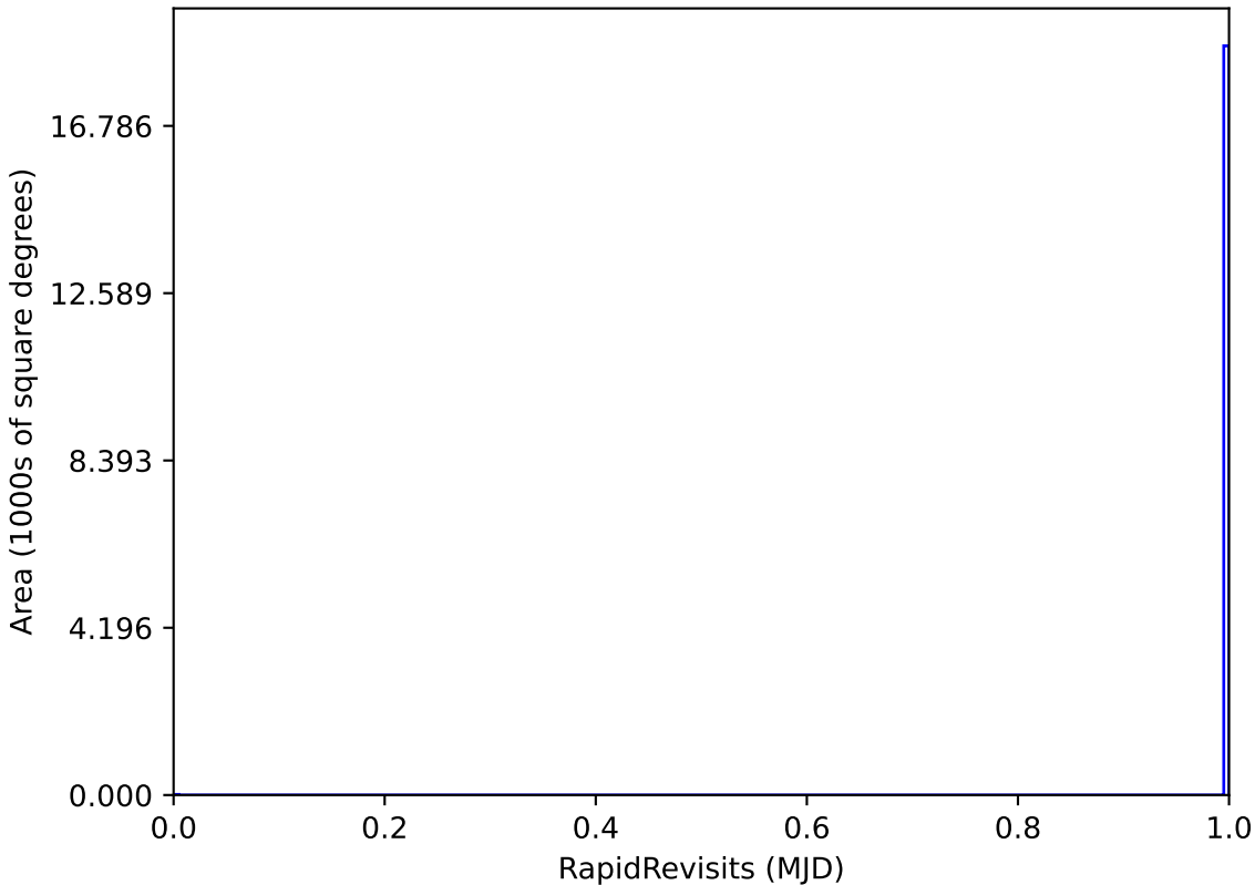
ddf_acor_sf10_lsf20_lsr50_v3.4_10yrs WFD: RapidRevisits
