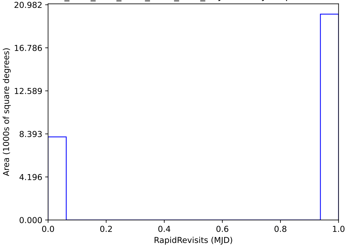
ddf_acor_sf10_lsf20_lsr50_v3.4_10yrs All sky: RapidRevisits
