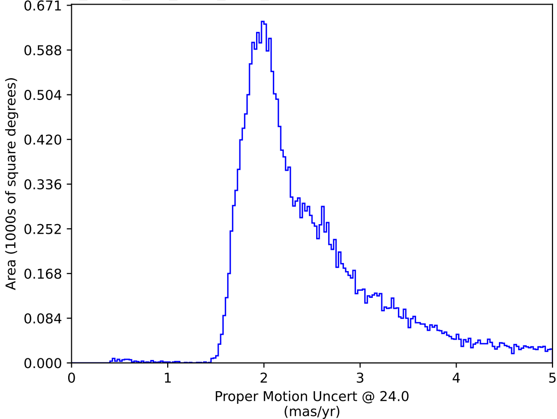
ddf_acor_sf10_lsf20_lsr50_v3.4_10yrs All sky: Proper Motion Uncert @ 24.0
