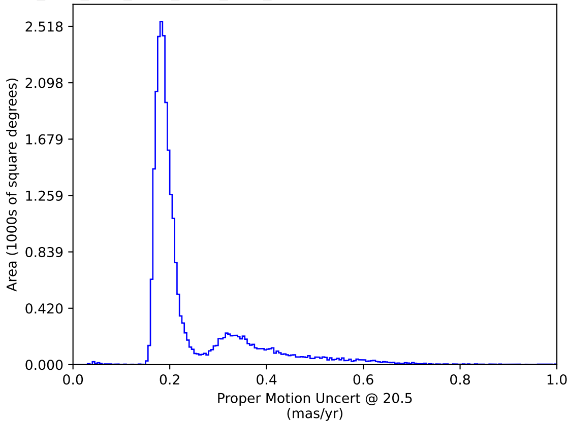
ddf_acor_sf10_lsf20_lsr50_v3.4_10yrs All sky: Proper Motion Uncert @ 20.5
