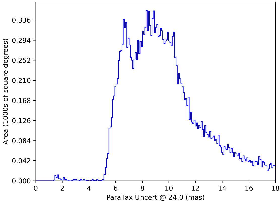
ddf_acor_sf10_lsf20_lsr50_v3.4_10yrs All sky: Parallax Uncert @ 24.0
