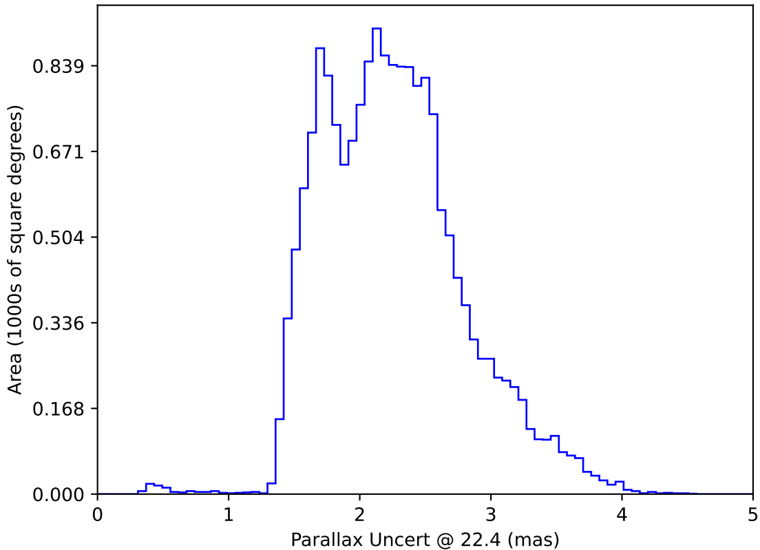
ddf_acor_sf10_lsf20_lsr50_v3.4_10yrs WFD: Parallax Uncert @ 22.4
