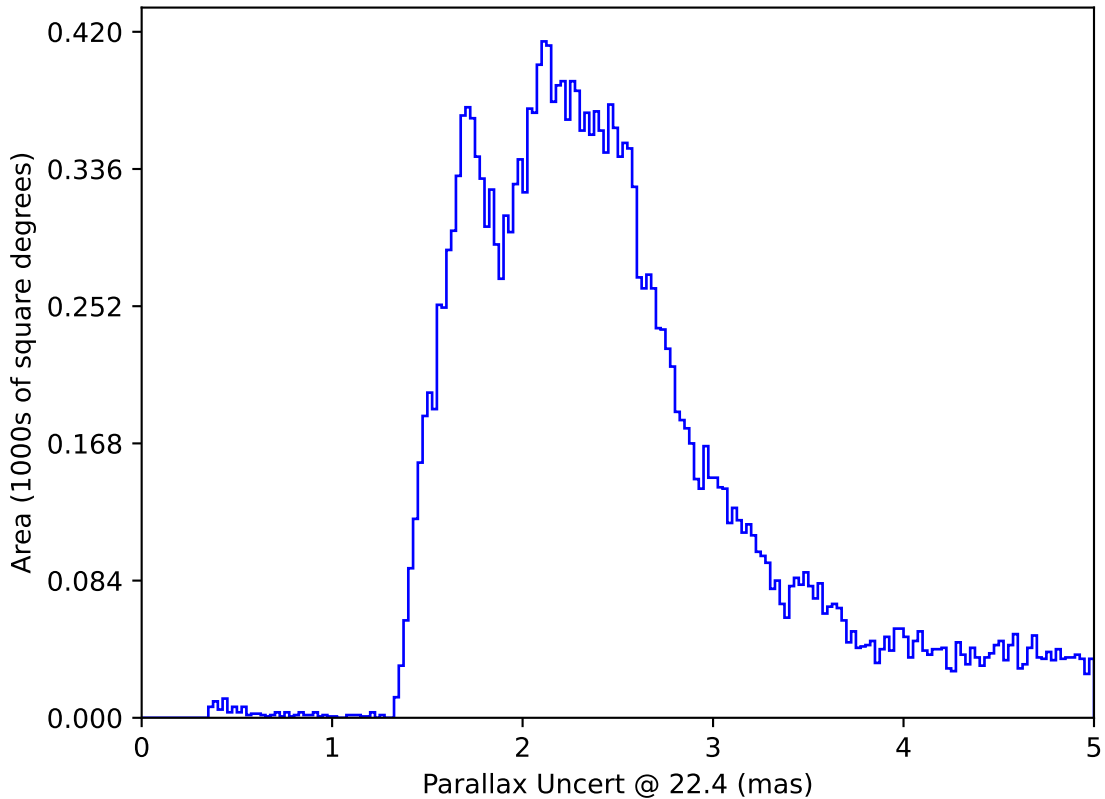
ddf_acor_sf10_lsf20_lsr50_v3.4_10yrs All sky: Parallax Uncert @ 22.4
